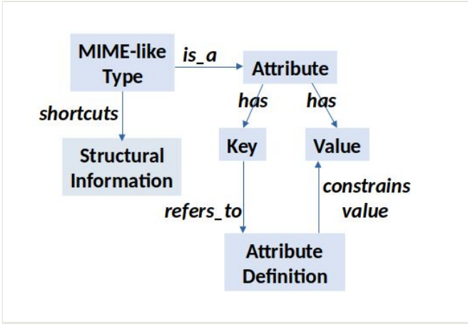
Figure 3. Community defined types similar to MIME types could be a light-weight way to enable operations on FDOs.
