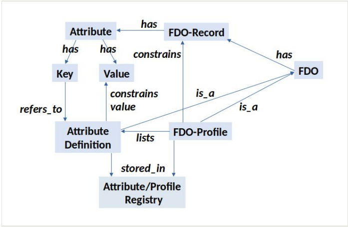
Figure 1. The FDO record determined by attribute definitions and profiles.
